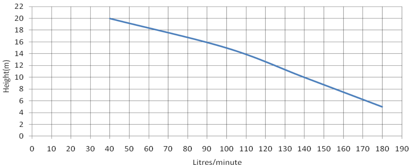
Pump Performance
